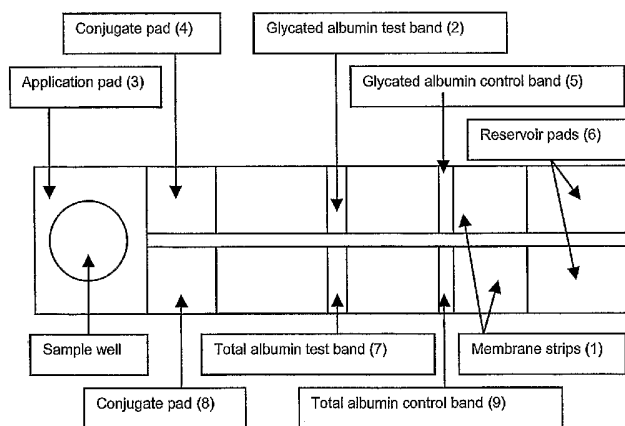
Test Strips: Overhead View
